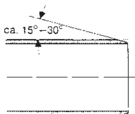
Figure 13. Chamfering in pipe ends.
