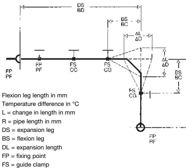
Figure 11. Installation using flexion legs.
