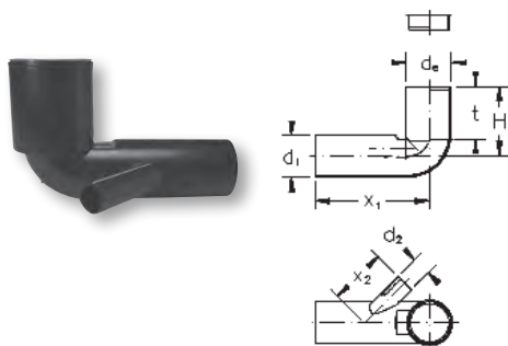
Long spigot toilet elbow with right stubs
